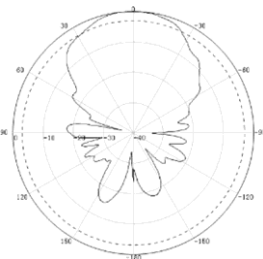
Vertical 1880MHz
