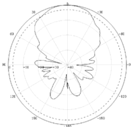
Vertical 1880MHz
