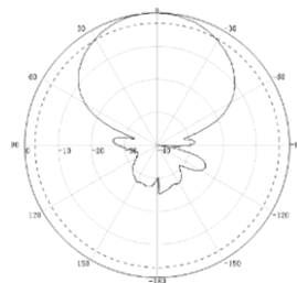
Vertical 960MHz
